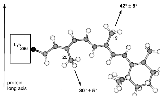
Fig. 3. Orientation and conformation of 11- cis retinal in the binding pocket of bovine rhodopsin in the ground state, constructed using the orientations of the methyl groups at the \text{C}_{19} and \text{C}_{20} position as determined by solid state ^2\text{H} NMR.
